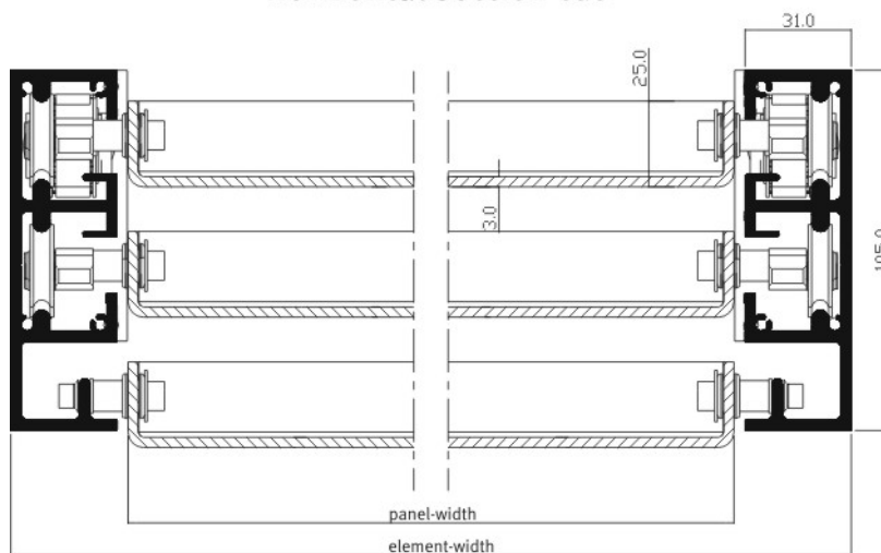
horizontal section cut
