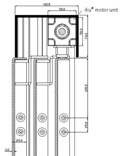
vertical section cut
